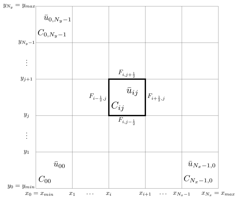
Figure 1: The Cartesian grid.
