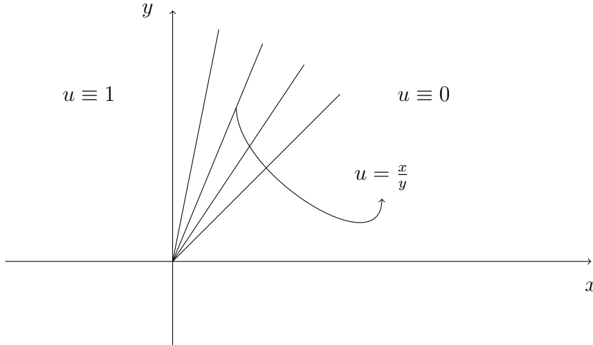
Figure 3.6: The expansion (or rarefaction) wave of Example 3.6.1 .
