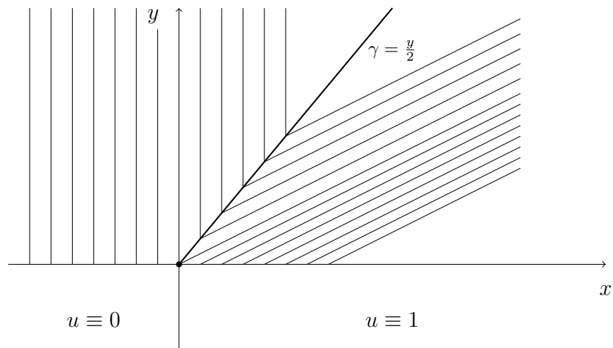
Figure 3.7: Characteristics emerging from the shock.
