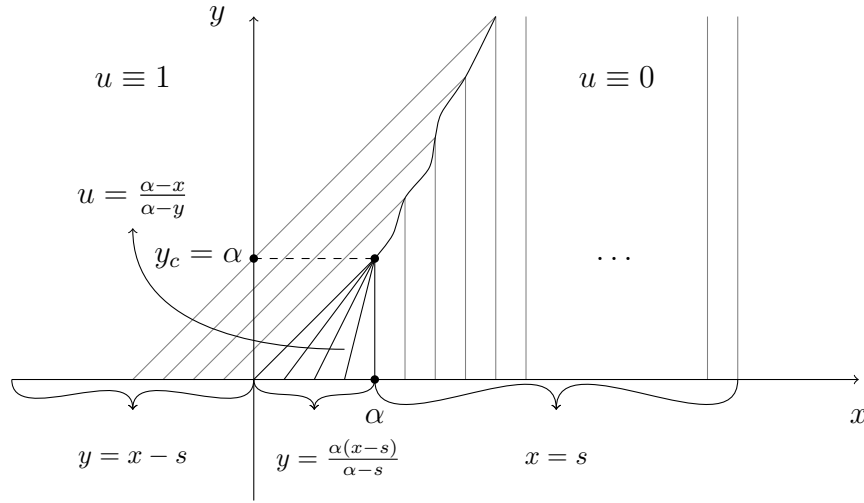
Figure 3.5: Intersection of characteristic curves in Example 3.6.1 .
